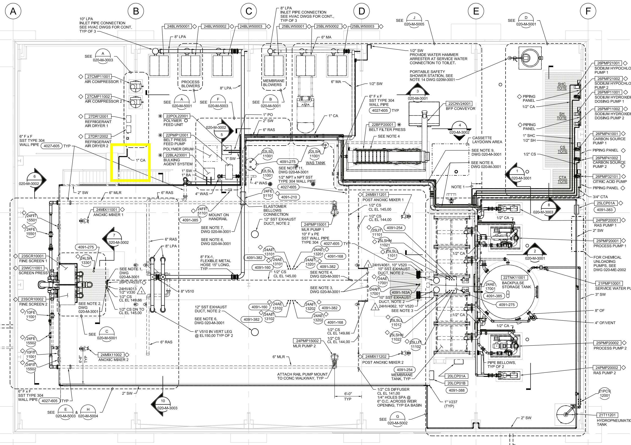
PLAN 3/16"=1'-0"
